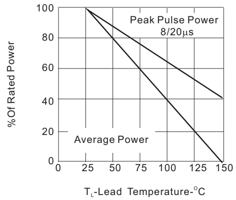
FIG. 2-Power Derating Curve
