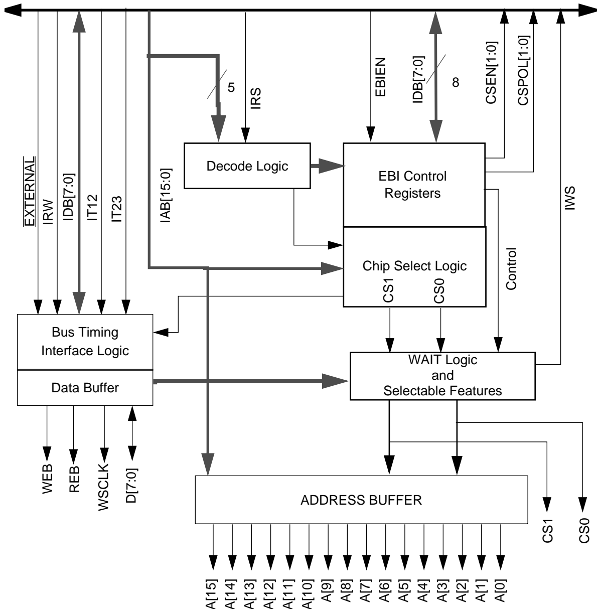
Figure 6 EBI Block Diagram
