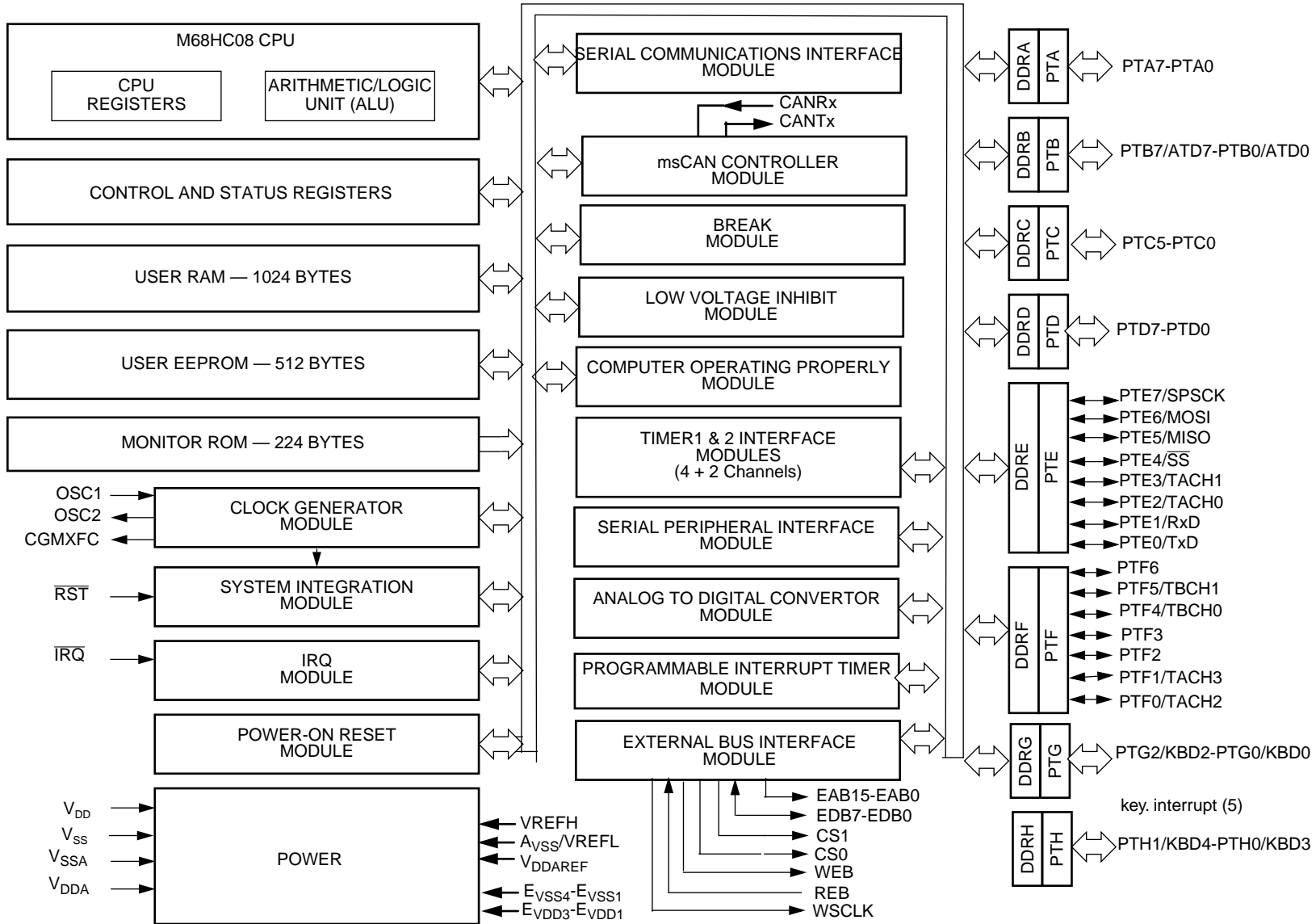
Figure 1. MC68HC08AZ0 MCU block diagram
