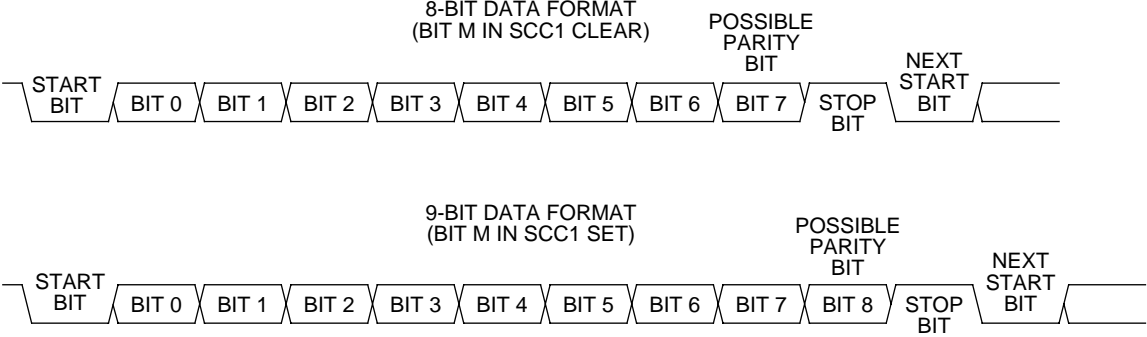
Figure 6. SCI data formats
