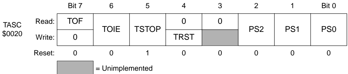
Figure 3. TIMA status and control register (TASC)
