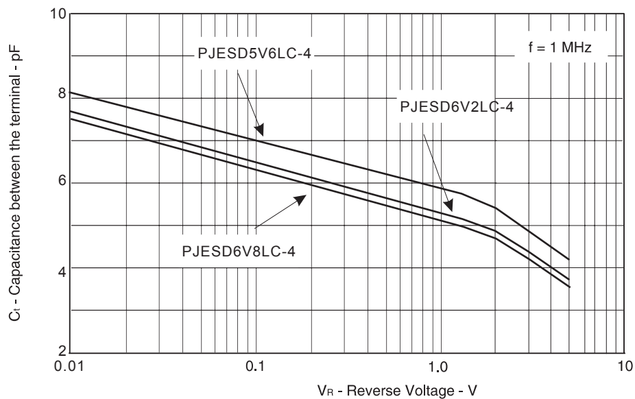
Figure 3.CT-VR CHARACTERISTICS
