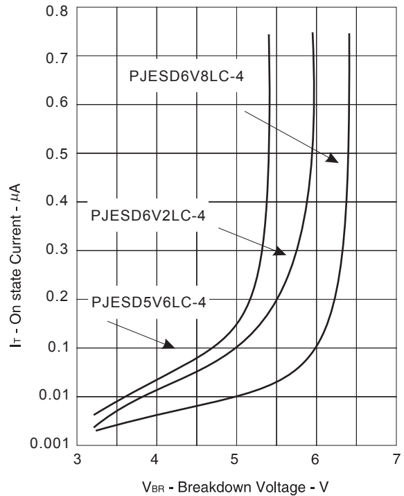
Figure 2.IT-VBR CHARACTERISTICS
