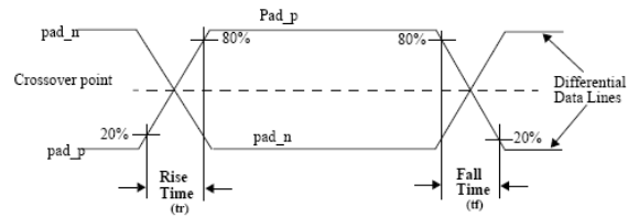
Figure 48. Rise/fall transition, part 1
