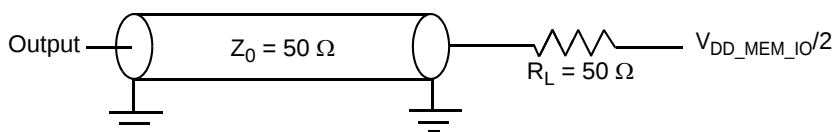
Figure 31. DDR AC test load
