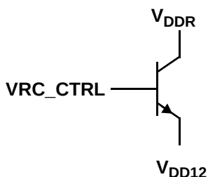
Figure 7. External NPN ballast connections
