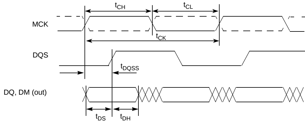
Figure 28. DDR write timing
