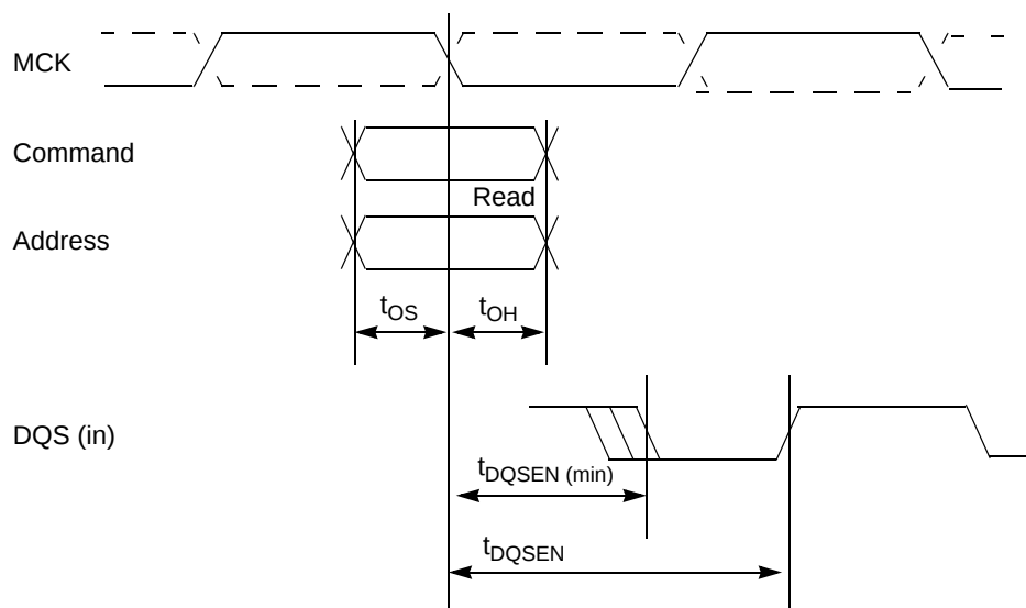
Figure 30. DDR read timing, DQSEN
