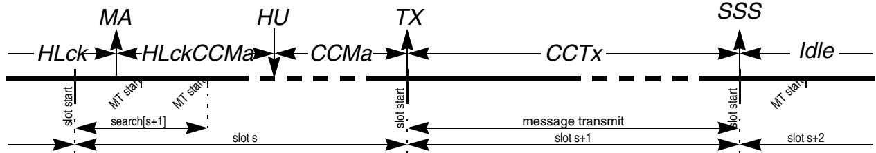
Figure 3-113. Message Transmission from HLck state with unlock
