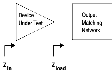
Figure 14. Series Equivalent Input and Load Impedance
