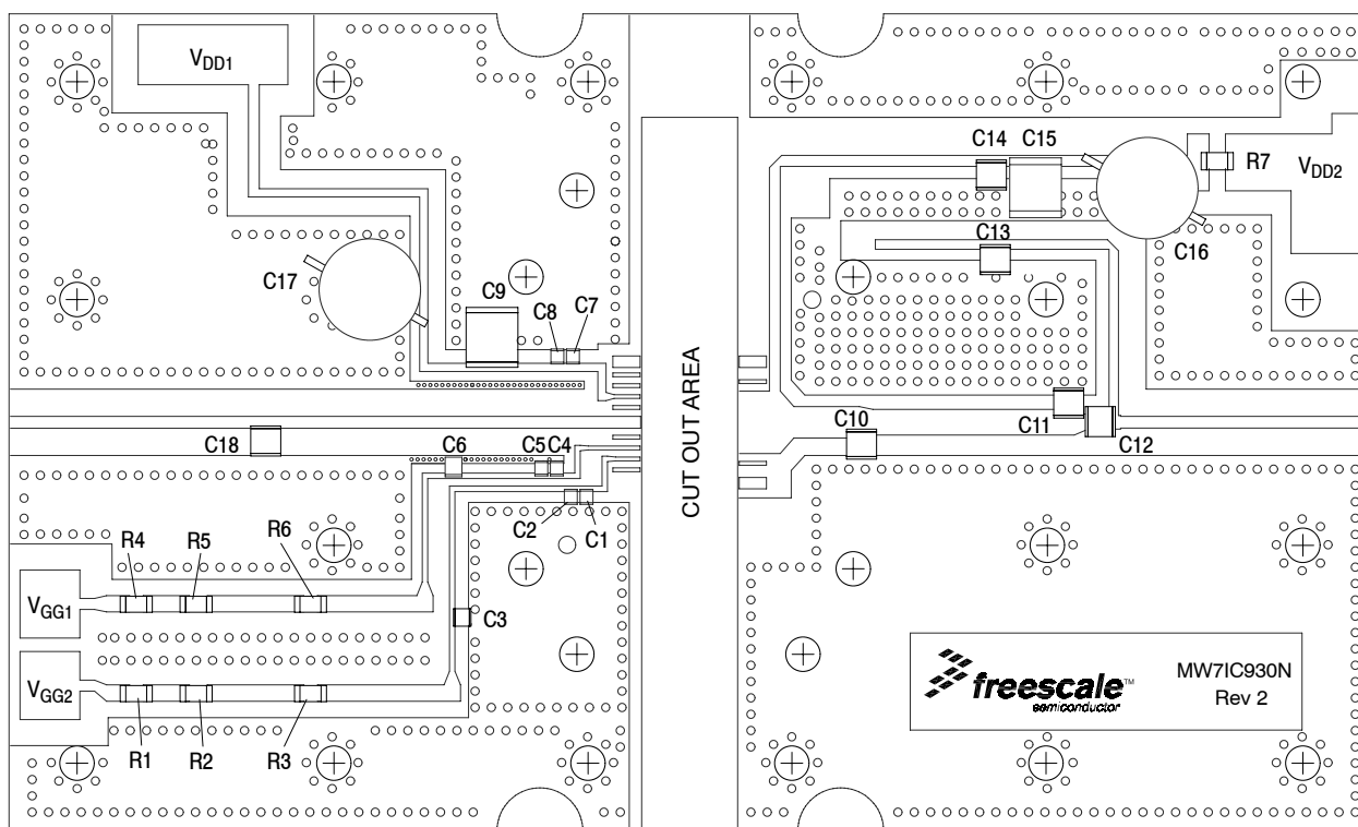
Figure 13. MW7IC930NR1(GNR1)(NBR1) Test Circuit Component Layout — 700 MHz
