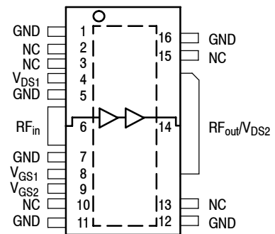
Figure 2. Pin Connections
