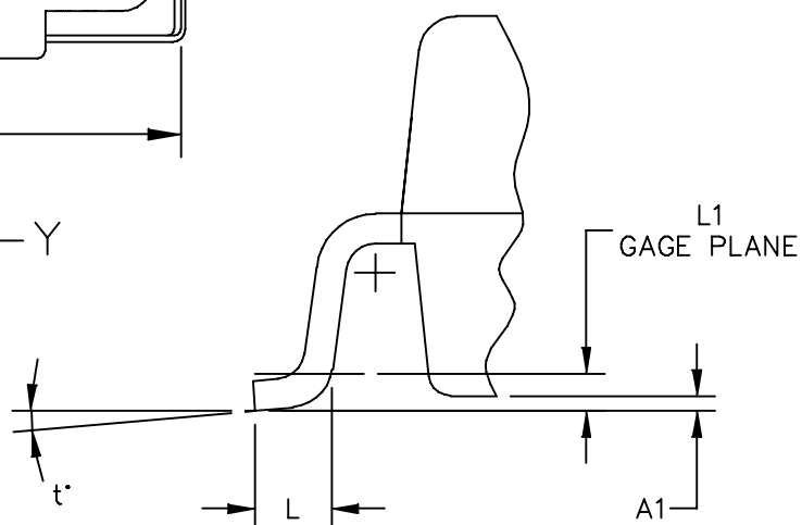
DETAIL "Y"
