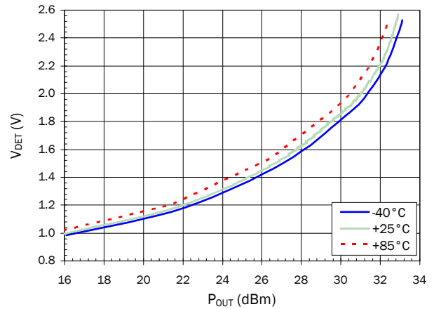
RF Power Detector ( V_{DET} ) versus P_{OUT} , F=3.7GHz
