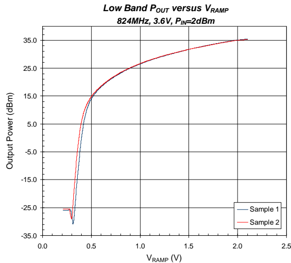
Figure 3. Graph of Output Power versus V_{\text{RAMP}}
