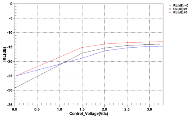
INPUT RETURN LOSS Vs. CONTROL VOLTAGE Vs. TEMPERATURE @ 806 MHz
