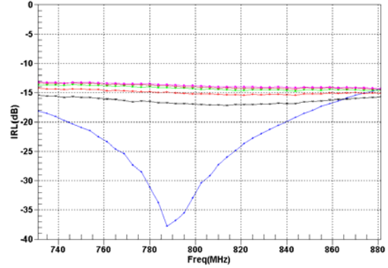
IRL Vs. FREQUENCY Vs. CONTROL VOLTAGE
