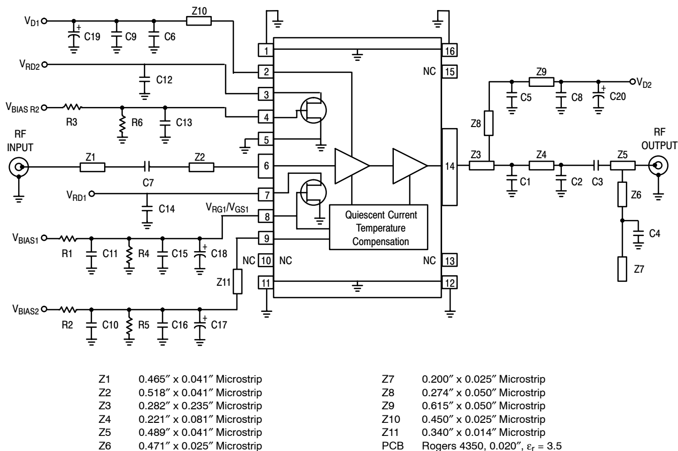
Figure 22. MW5IC2030MBR1(GMBR1) Test Circuit Schematic for Driver Application Tests
