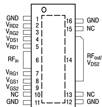
CASE 1329A-03 TO-272 WB-16 GULL PLASTIC MW4IC915GNBR1
