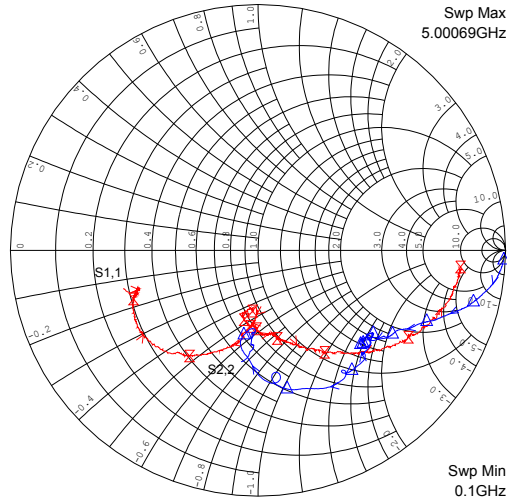
Smith Chart
