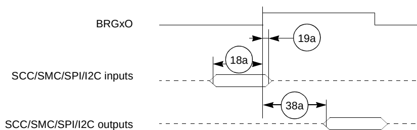
Figure 2-20. SCC/SMC/SPI/I²C Internal Clock Diagram
