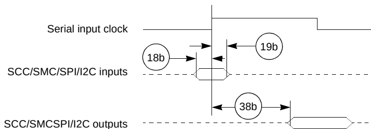
Figure 2-21. SCC/SMC/SPI/I²C External Clock Diagram
