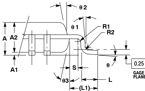
DETAIL F
