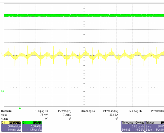
Typical Output Ripple at 48V Input and Full Load at Ta=25C Ch. 1: Vo Ch. 4: Io
