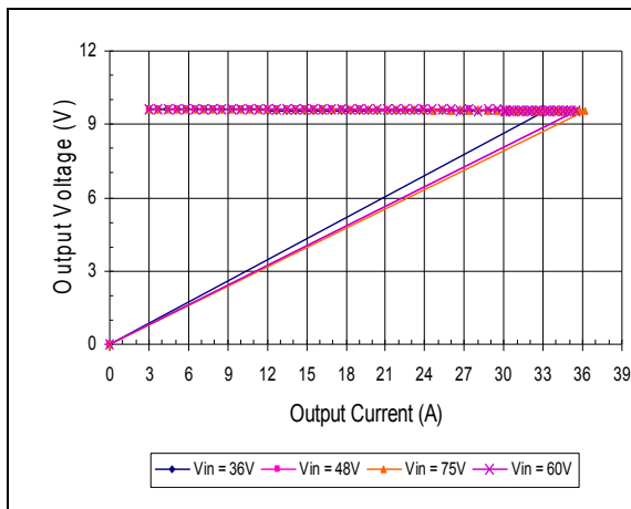
Typical Output Current Limit vs. Input Voltage
