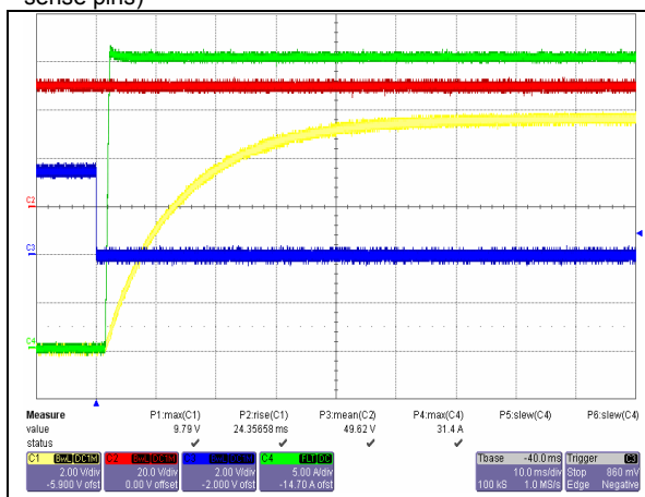
Start-up from on/off Switch at 48V input and Full Load. Ch. 1: Vo Ch. 2: Vin Ch. 3: ON/OFF Ch. 4: Io
