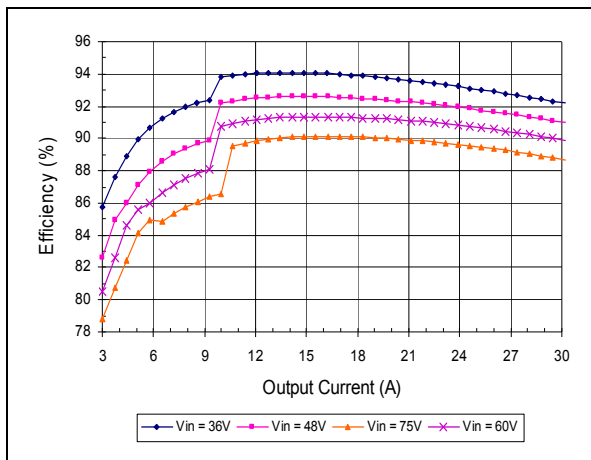
Efficiency vs. Input Voltage (test in socket w/o remote sense pins)
