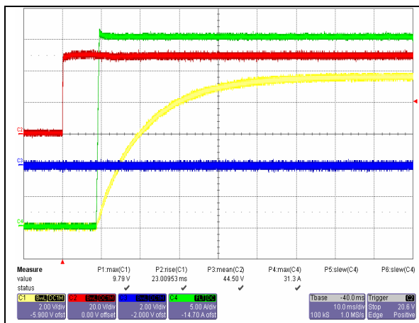
Start-up from Input Voltage Application at Full Load. Ch. 1: Vo Ch. 2: Vin Ch. 3: ON/OFF Ch. 4: Io
