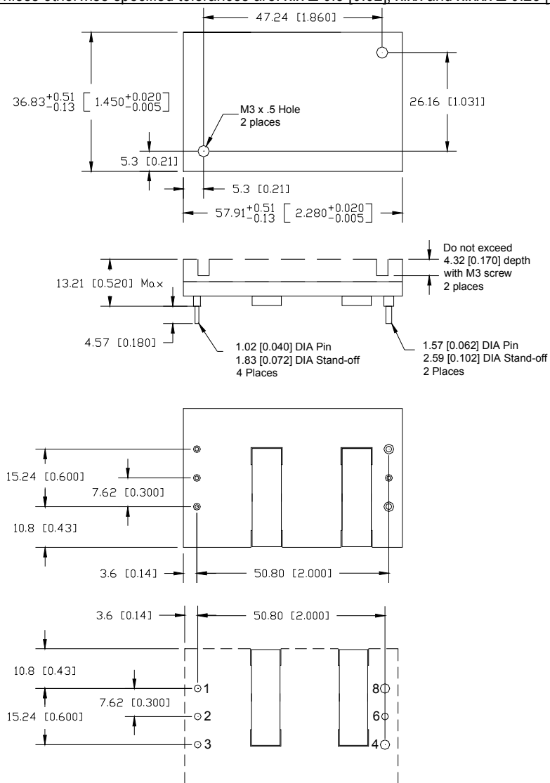
Recommended hole pattern (top view)
