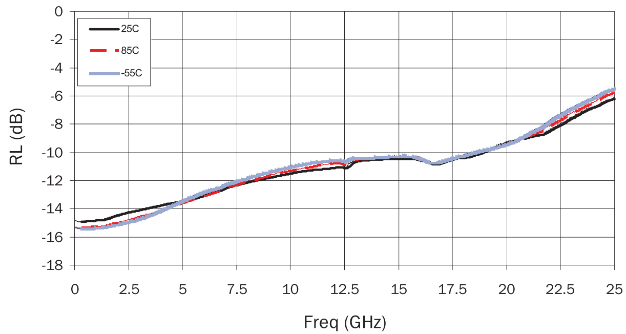
Input Return Loss vs. Temp (RFO off , Vcontrol = -5V)
