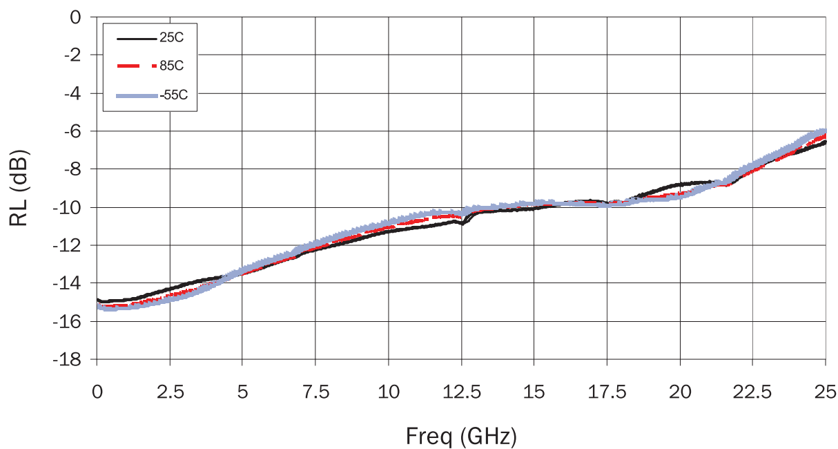
Output Return Loss vs. Temp (RFOff, Vcontrol = -5V)
