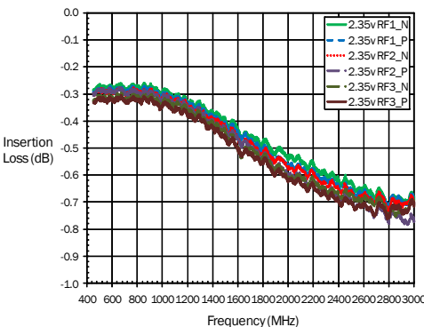
Max Insertion Loss (Temp=25 °C, VRF=2.35V)
