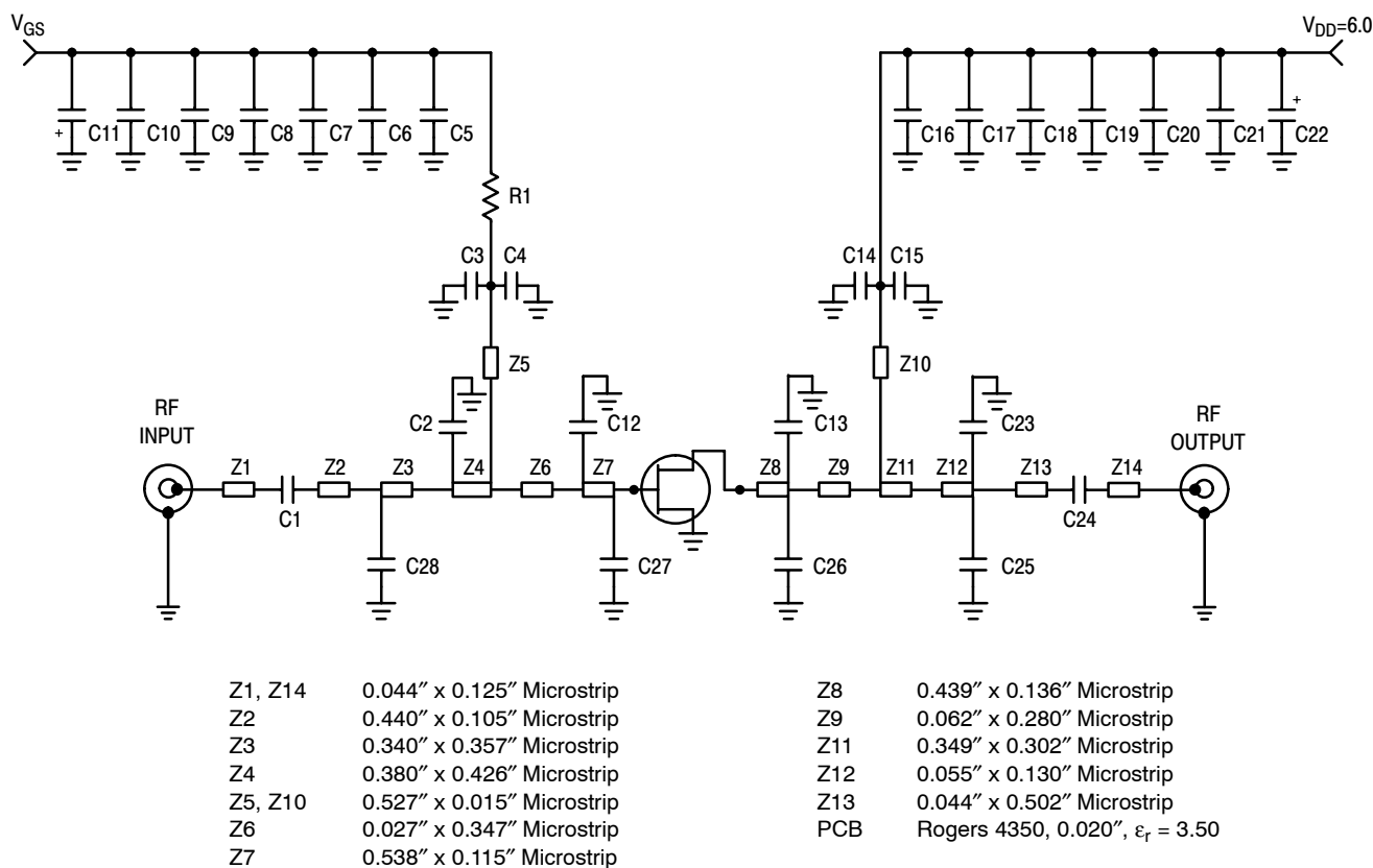
Figure 1. 3.5 GHz Test Circuit Schematic
