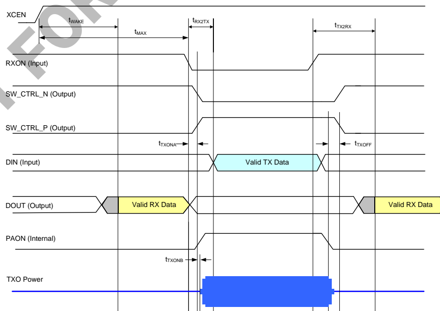
Figure 2 Control Timing for TDD Operation, PAFIRST=0 (The external switch controls SW_CTRL_P/N are switched before PA is turned on).
