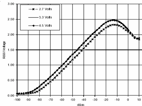
Figure 2a. RSSI Output Voltage vs Input Signal Level (Unclicked, 25°C, Various Input Voltage Levels)
