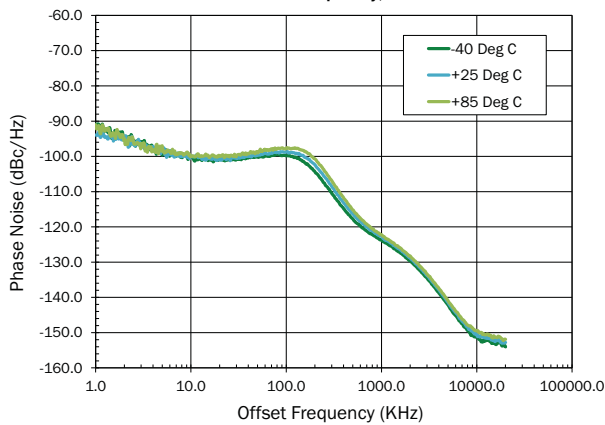
Synthesizer Phase Noise vs Temperature 2000MHz LO Frequency, 26MHz TCXO
