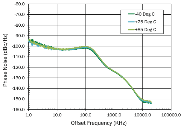
Synthesizer Phase Noise vs Temperature 1500MHz LO Frequency, 26MHz TCXO
