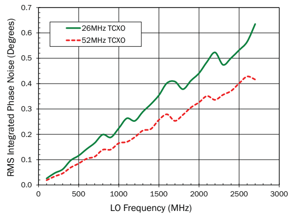
Synthesiser RMS Integrated Phase Noise Integration Bandwidth 1KHz to 40MHz
