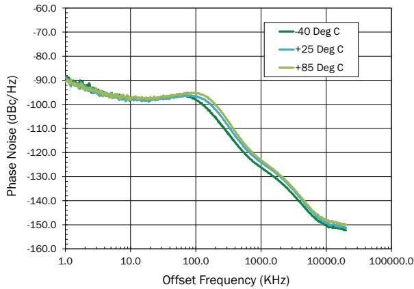
Synthesizer Phase Noise vs Temperature 2600MHz LO Frequency, 26MHz TCXO
