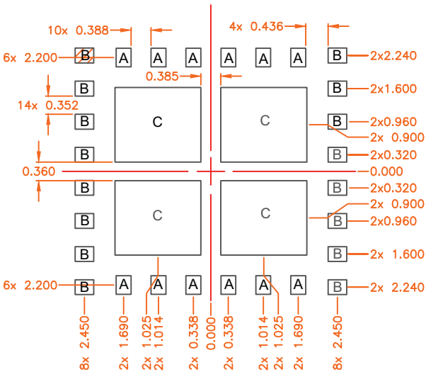
PCB Stencil Pattern
