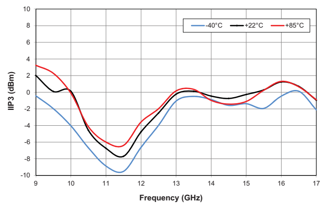
IIP3 (dBm) vs. RF Freq, Over Temperature
