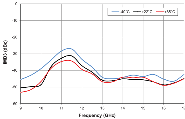
IMD3 (dBc) vs. RF Freq, Over Temperature
