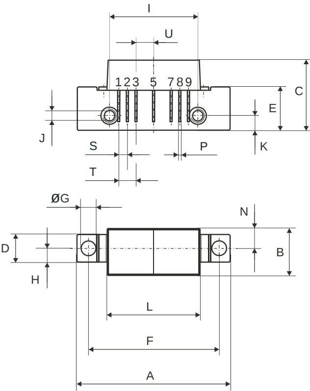
Pinning:
