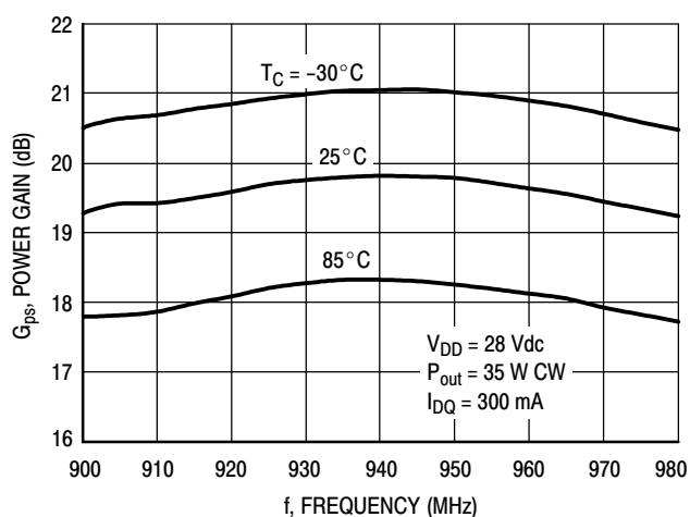
Figure 13. Power Gain versus Frequency
