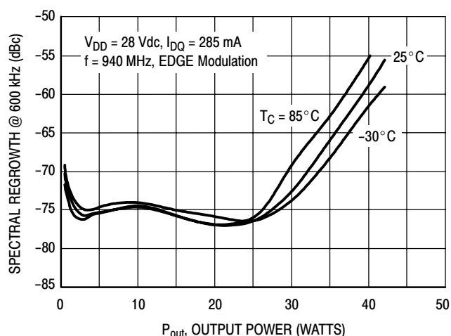
Figure 11. Spectral Regrowth at 600 kHz versus Output Power
