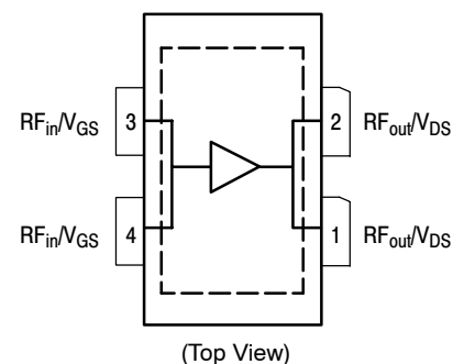
Figure 1. Pin Connections
