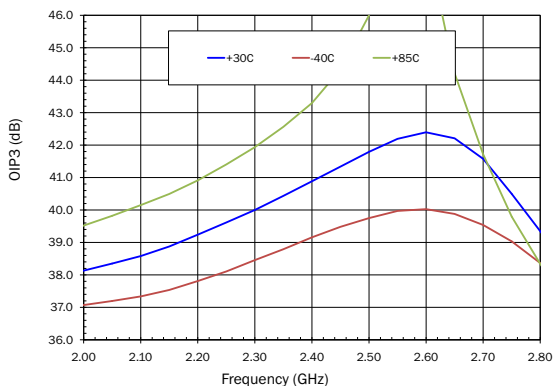
Output IP3 versus Frequency
