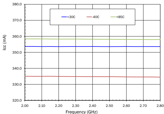
Current versus Frequency
