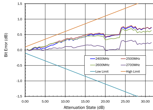
Bit Error versus Attenuation State
