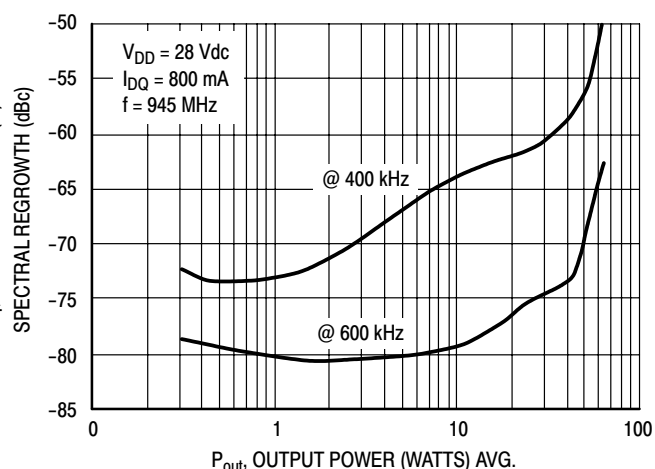
Figure 10. Spectral Regrowth versus Output Power
