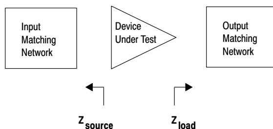
Figure 13. Series Equivalent Source and Load Impedance (MRF9045MBR1)
