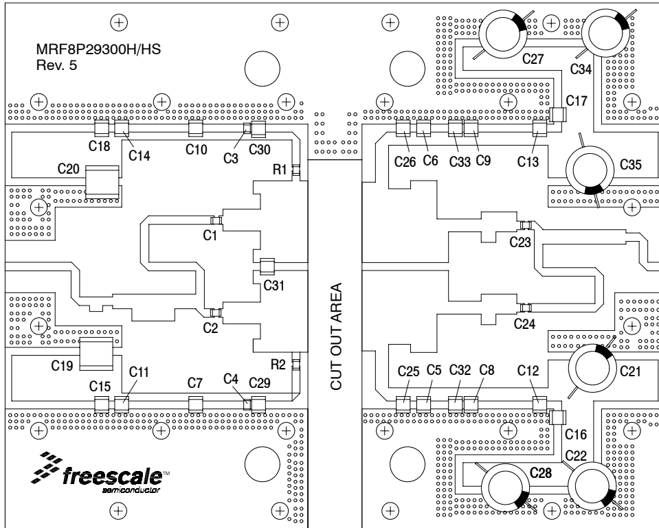
Figure 3. MRF8P29300HR6(HSR6) Test Circuit Component Layout
