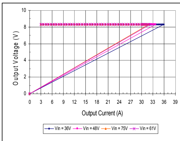
Typical Output Current Limit vs. Input Voltage
