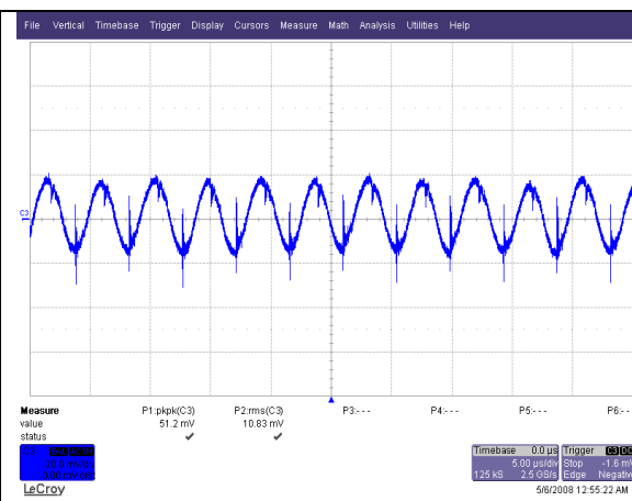
Typical Output Ripple at 48V Input and Full Load at Ta=25C Ch. 3: Vo
