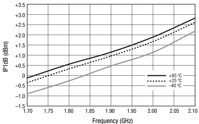
Figure 9. IP1dB vs Frequency Over Temperature
