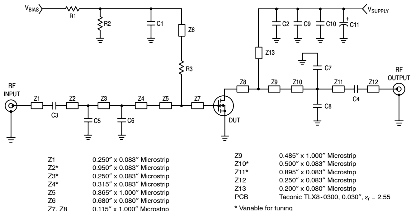
Figure 1. MRF6S18060MR1 (MBR1) Test Circuit Schematic — 1900 MHz
