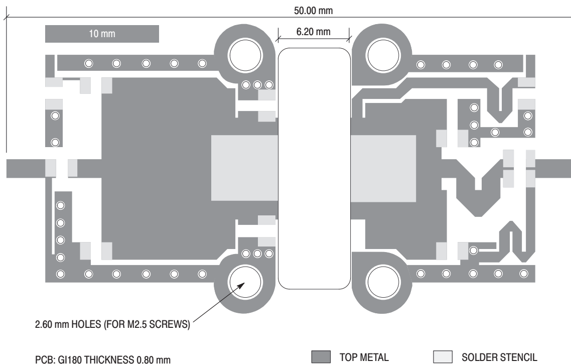
Figure 10. PCB Layout
