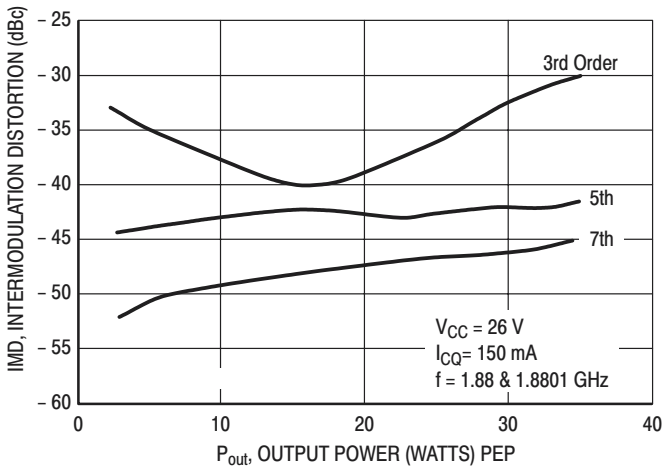
Figure 4. Intermodulation versus Output Power
