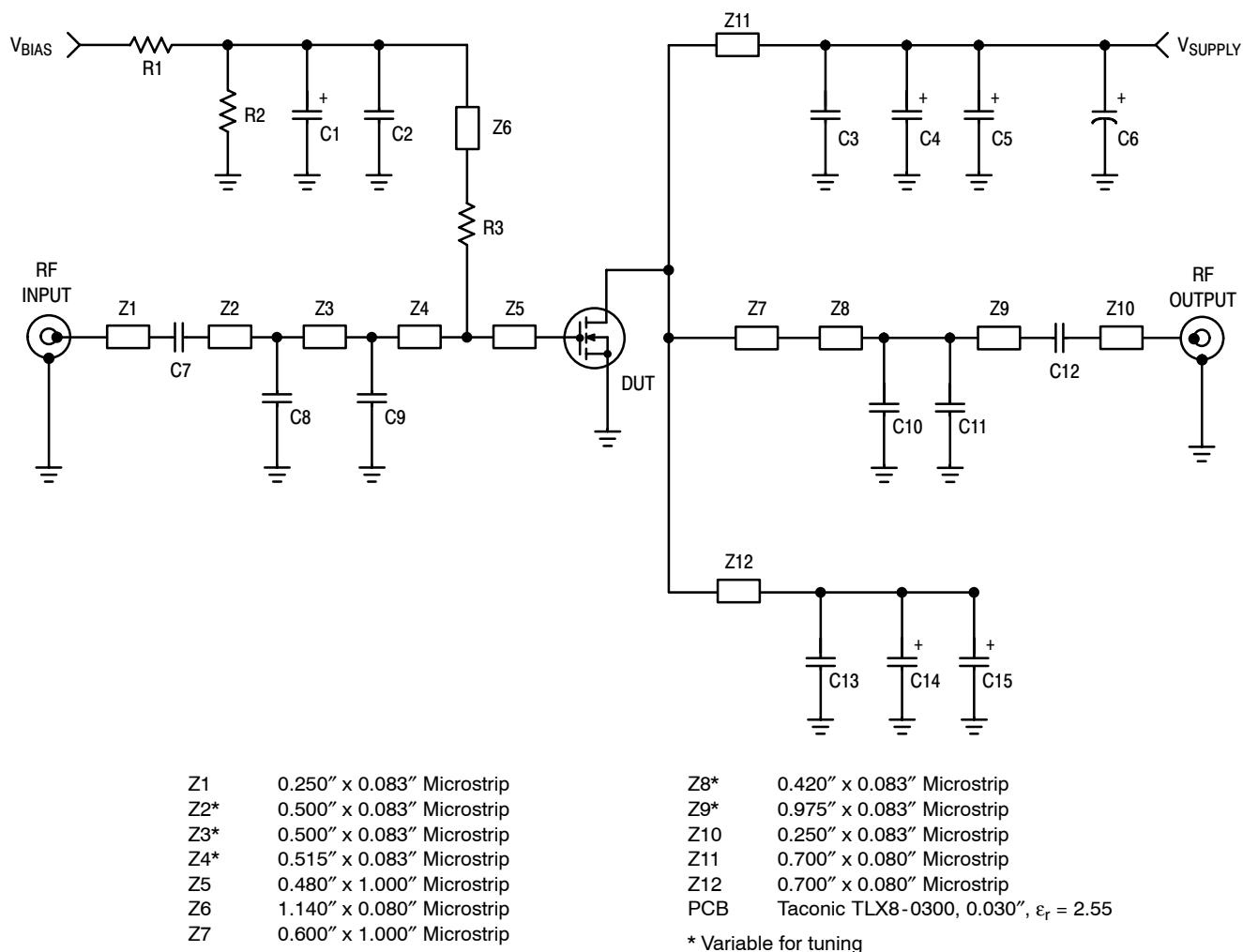
Figure 1. MRF5S19060MR1/MBR1 Test Circuit Schematic
