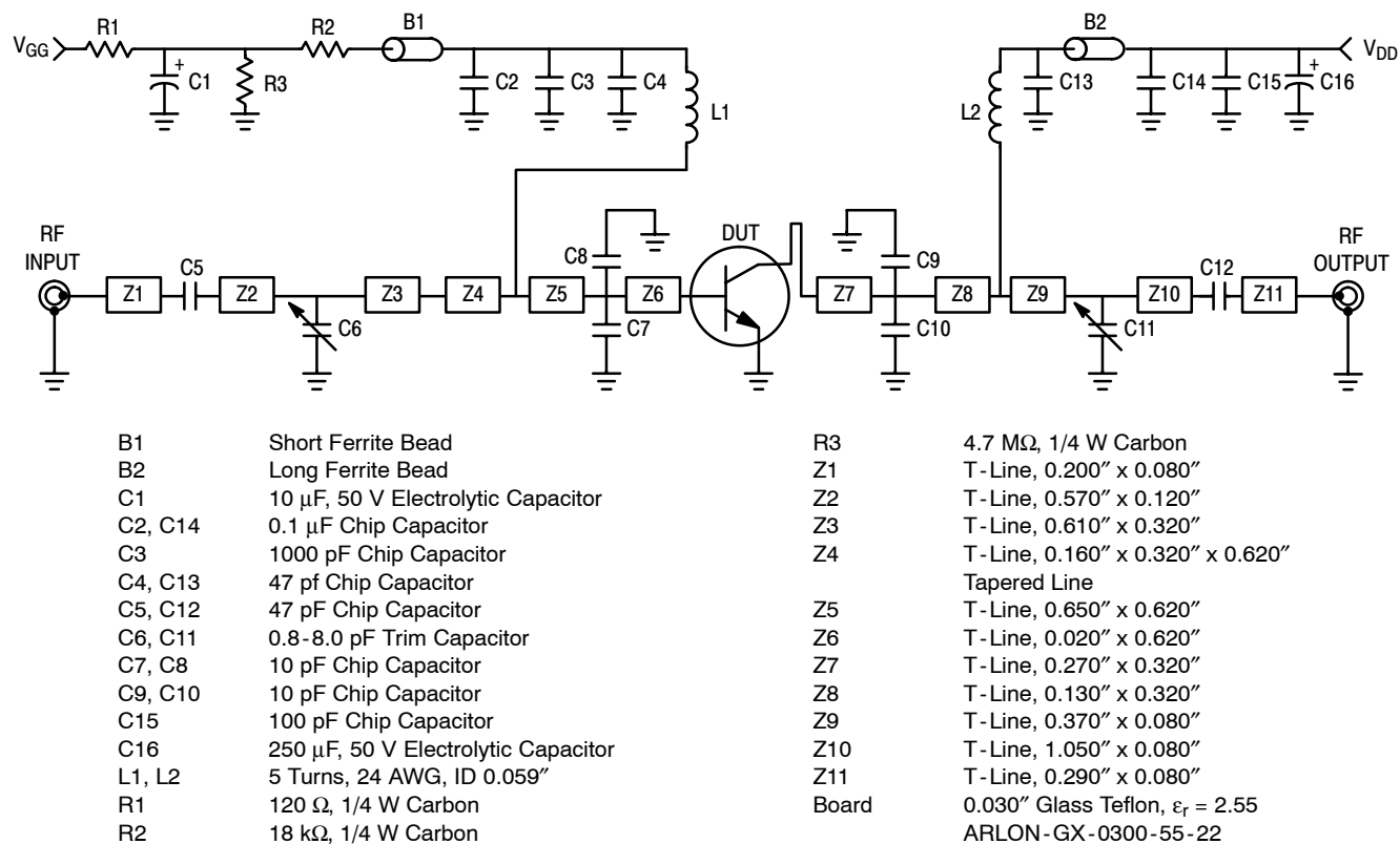
Figure 1. MRF183LSR1 Two Tone Test Circuit Schematic
