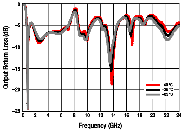
Figure 11. Small Signal Output Return Loss (IS22) vs Frequency and Temperature, Wide Band
