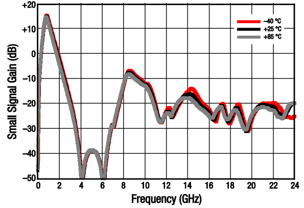
Figure 8. Small Signal Gain (IS21) vs Frequency and Temperature, Wide Band
