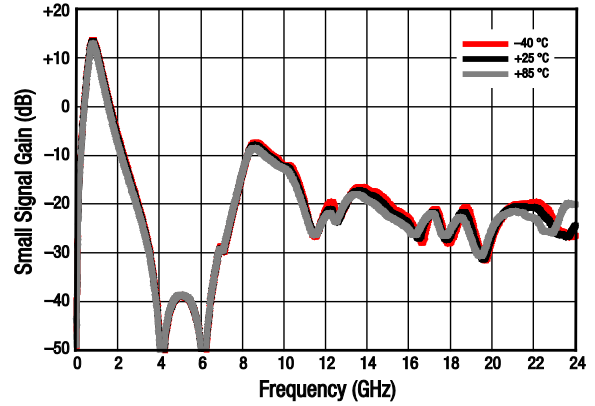
Figure 21. Small Signal Gain (IS21I) vs Frequency and Temperature, Wide Band
