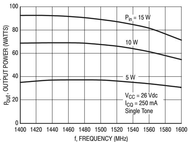
Figure 2. Output Power versus Frequency
