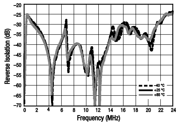
Figure 23. Small Signal Reverse Isolation (IS12I) vs Frequency and Temperature, Wide Band
