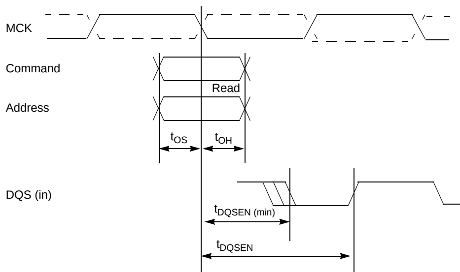
Figure 33. DDR read timing, DQSEN
