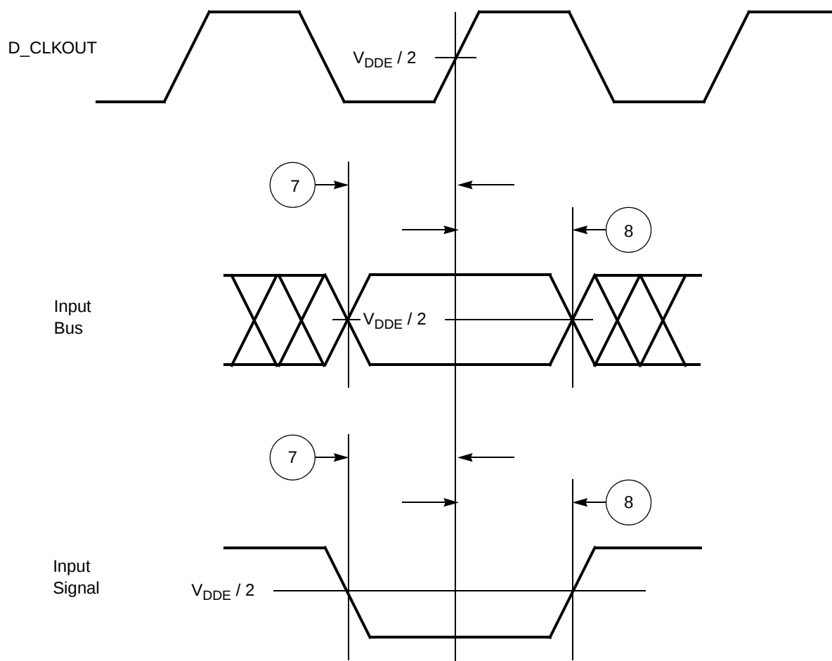
Figure 57. Synchronous input timing
