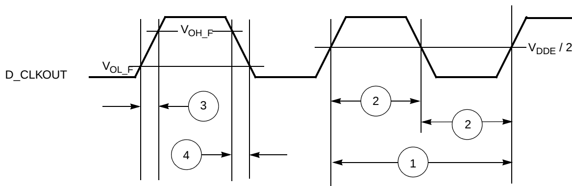
Figure 55. D_CLKOUT timing
