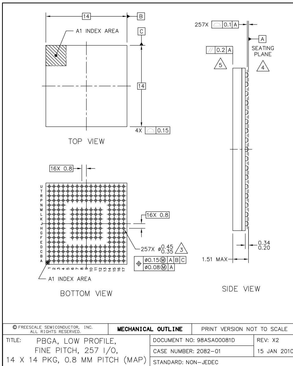
Figure 60. 257 MAPBGA mechanical data (1 of 2)
