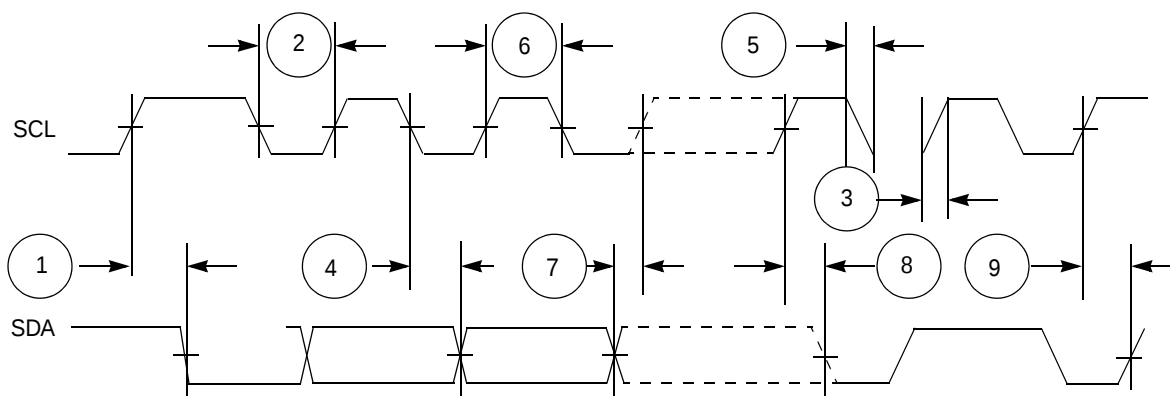
Figure 59. I²C input/output timing
