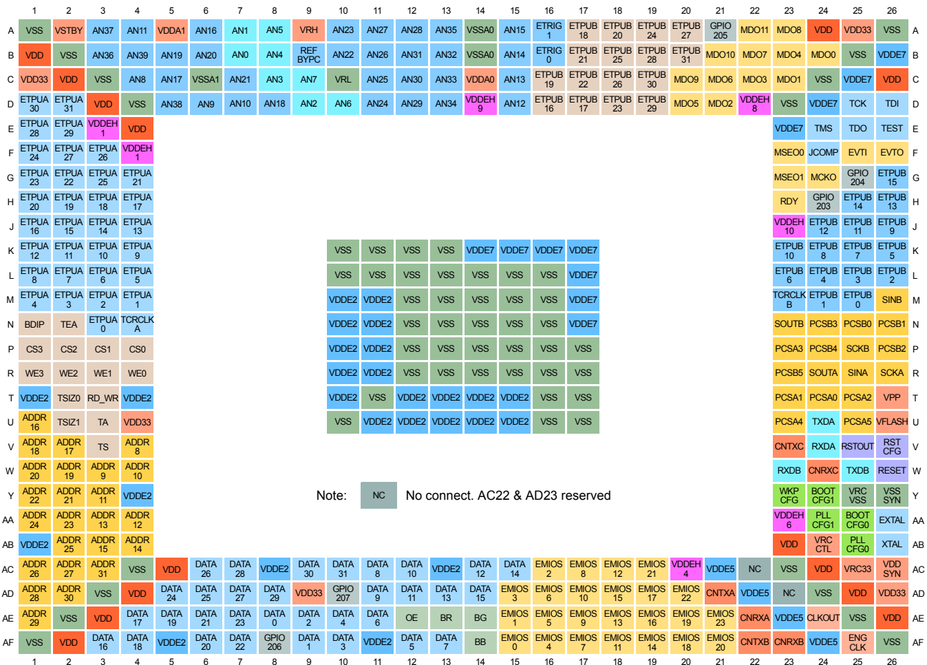
Figure 32. MPC5566 416 Package
