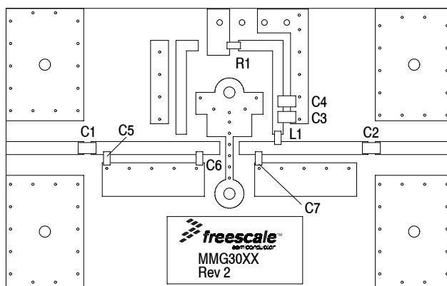
Figure 25. 50 Ohm Test Circuit Component Layout
