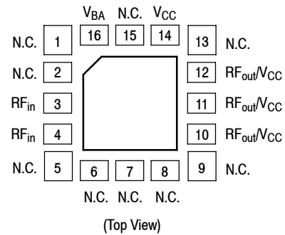
Pin Connections
