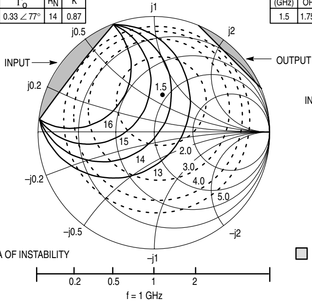
Figure 18. MRF947 Series Constant Gain and Noise Figure Contours
