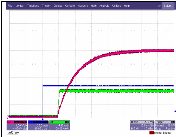
Start-up from Input Voltage Application at Full Load. Ch. 2: Vo Ch. 3: Vin Ch. 4: Io
