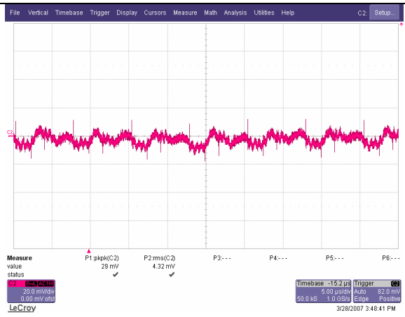
Typical Output Ripple at 48V Input and Full Load at Ta=25°C Ch. 2: Vo
