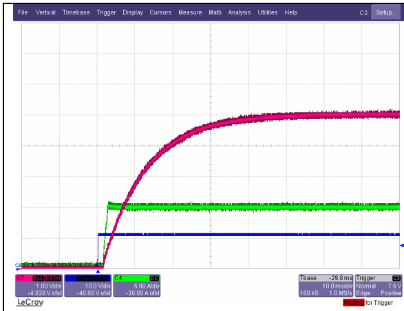
Start-up on on/off Switch at 48V input and Full Load. Ch. 2: Vo Ch. 3: ON/OFF Ch. 4: Io
