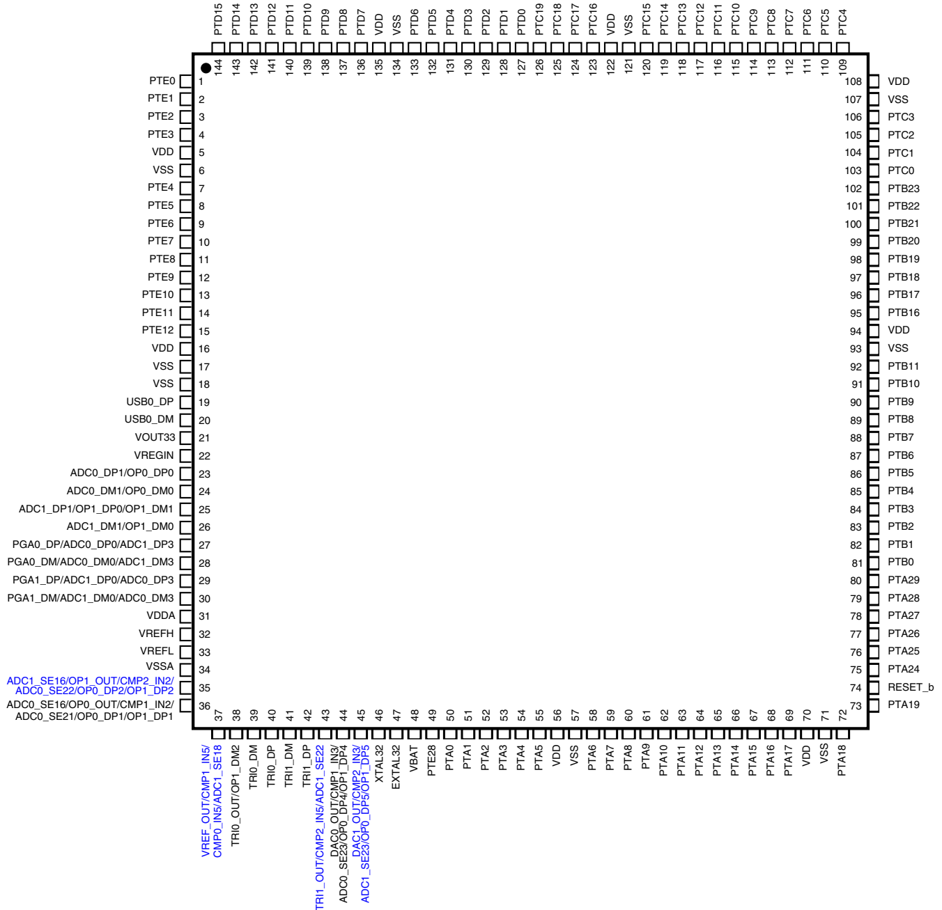
Figure 29. K52 144 LQFP Pinout Diagram
