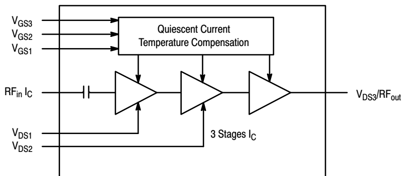
Figure 1. Block Diagram
