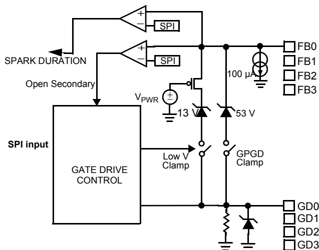
Figure 8. Low-voltage Clamp
