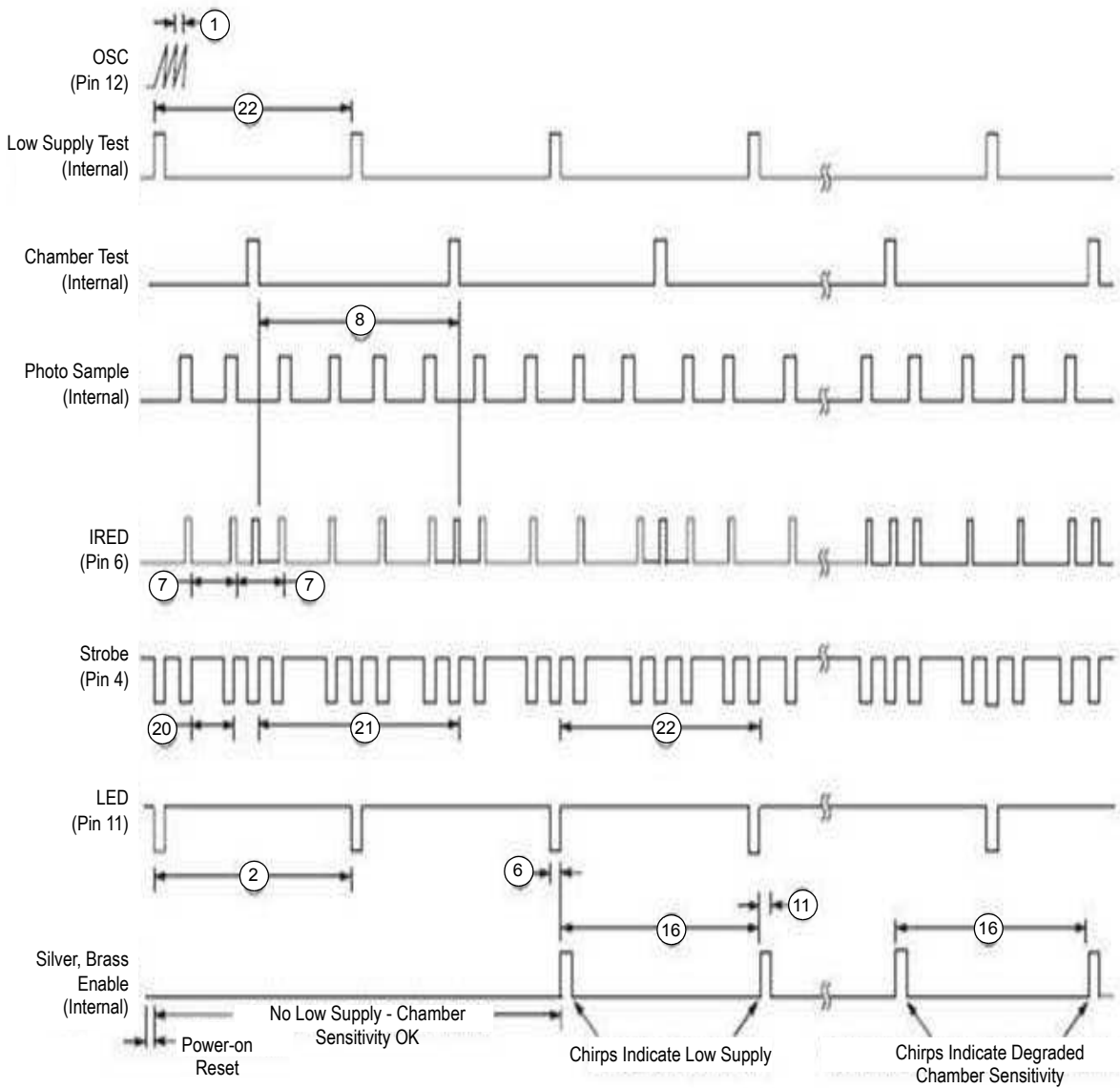
Figure 3. Typical Standby Timing Diagram MC146012 Device
